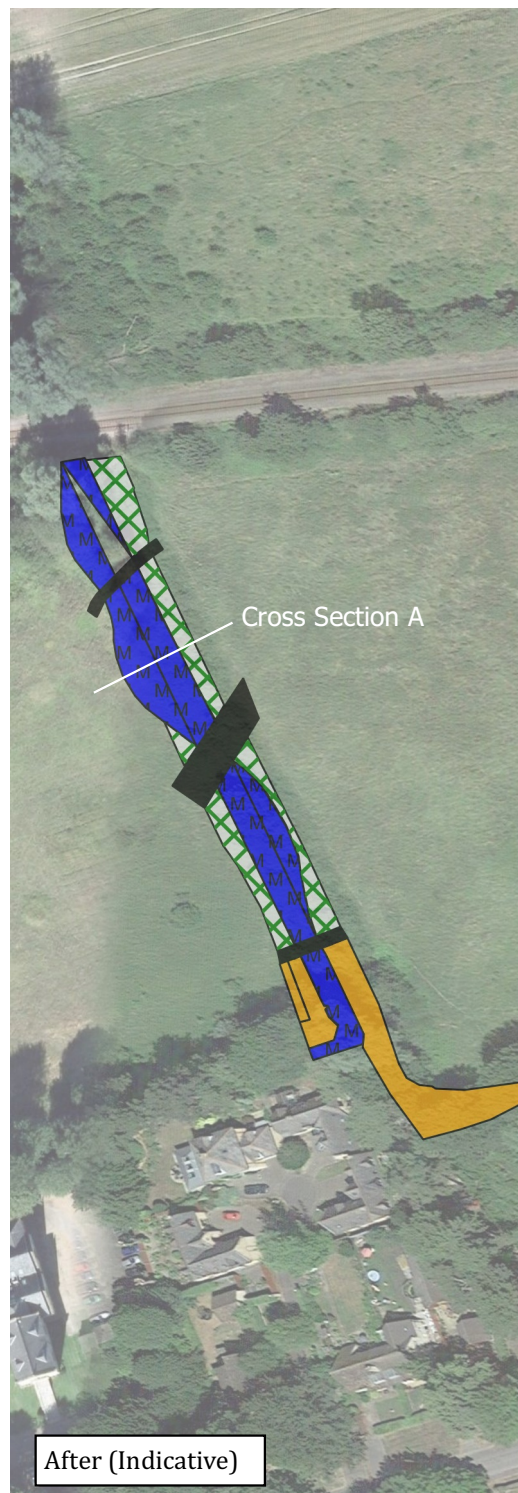
Indicative illustration of the revised chalk stream channel at Cross Section A following modification works.
