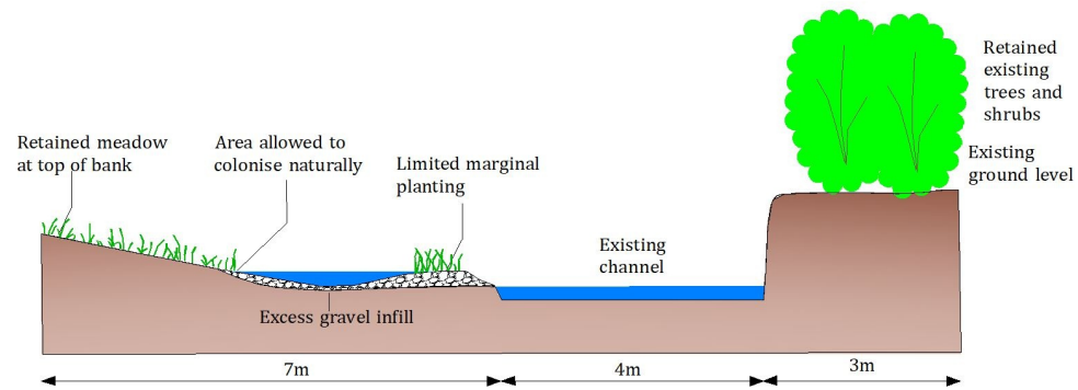
Indicative illustration of the revised chalk stream channel at Cross Section A following modification works.
