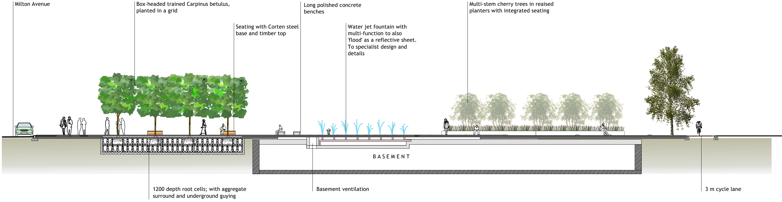
S-1 Chesterton Square long section Scale 1:200 @ A3
