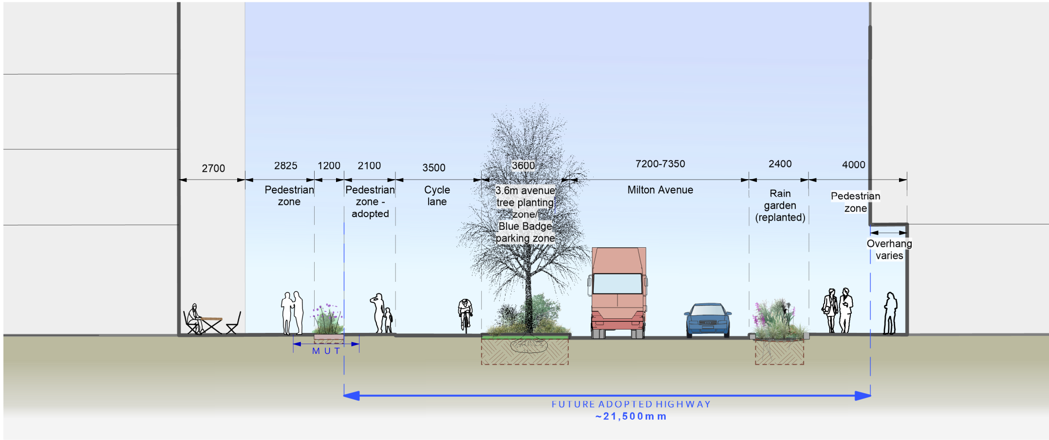
S-1 Milton Avenue- Section A-A Scale 1:150 @ A3
