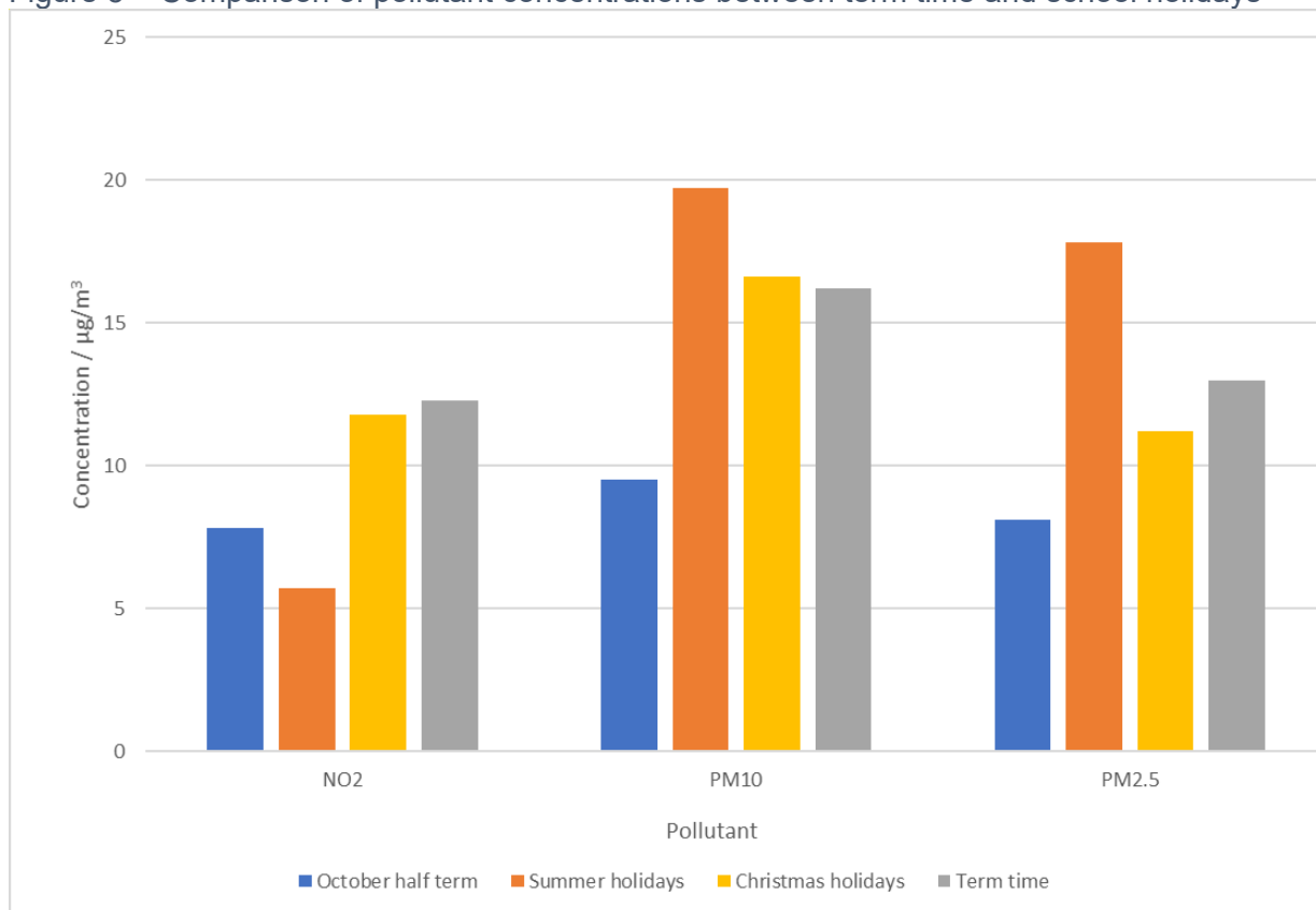
Figure 5 – Comparison of pollutant concentrations between term time and school holidays
