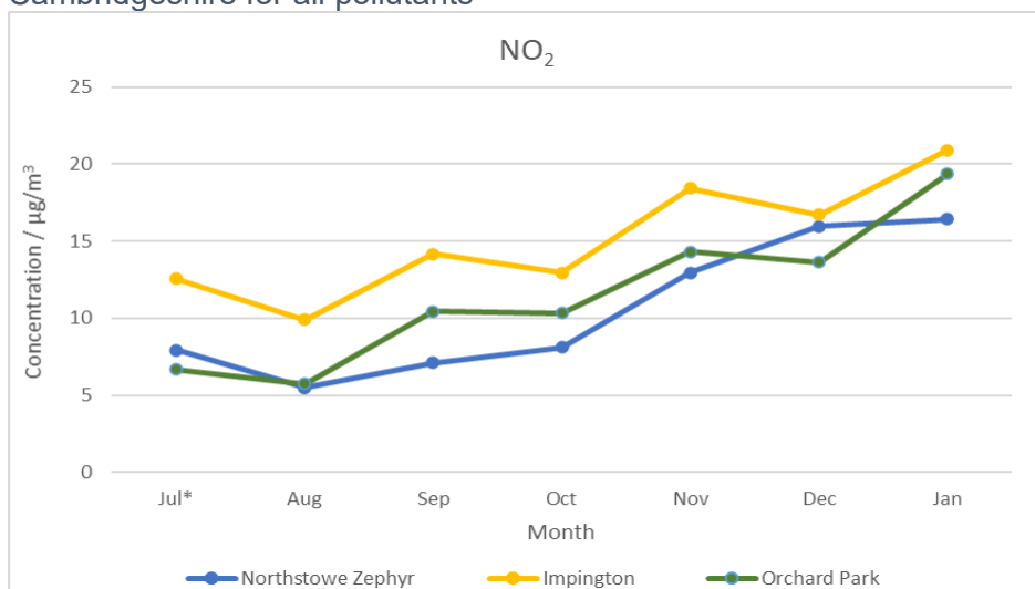
Figure 4. Comparison of Northstowe Zephyr data to automatic monitoring sites in South Cambridgeshire for all pollutants
